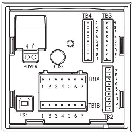
1/4 DIN housing (panel mount)
