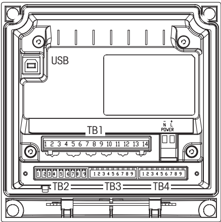
1/2 DIN housing (wall mount)
